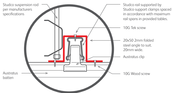
Detail C: Z Bracket
