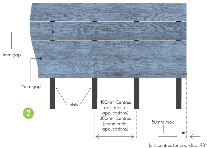
Joist centres for boards at 90°
