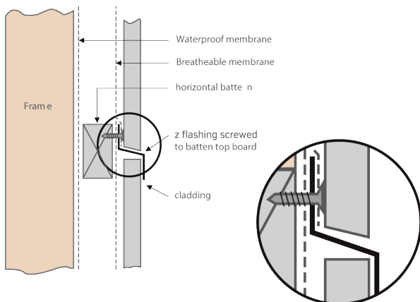
Expansion Gap Detail A Vertical installation
