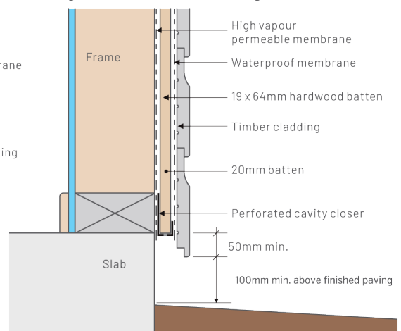
Minimum clearance of cladding above final ground levels and finishing below bottom
