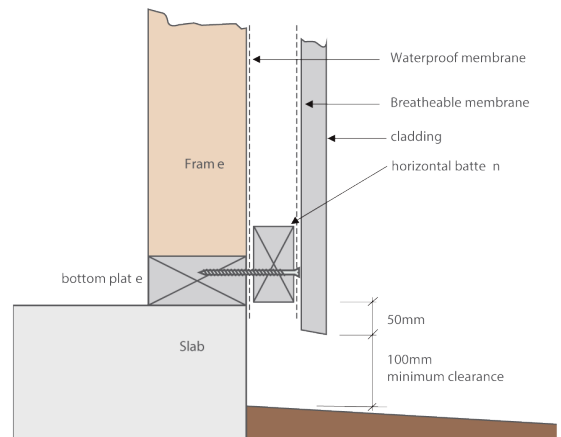
Bottom Edge – Detail B Vertical installation
