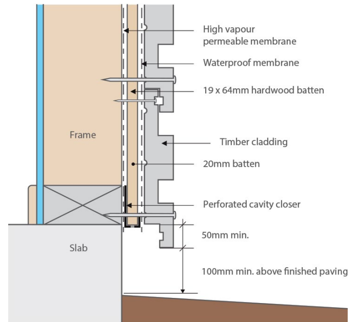
Horizontal installations - external
