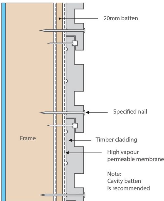
Face fixing showing fixing position
