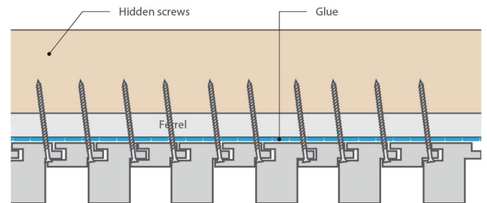
Horizontal installation - internal ceiling
