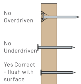
Figure 3: Nail Driving detail
