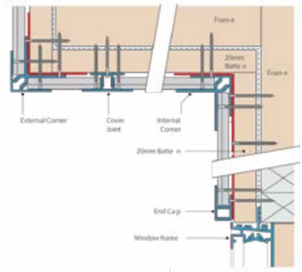
Internal / external stops (Aluminium) Note: Nail or Screw cladding as specified
