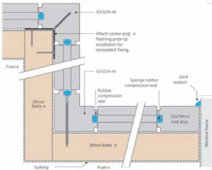
Internal / external stops (timber)
