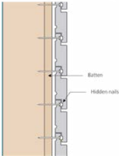
Horizontal installation – internal wall
