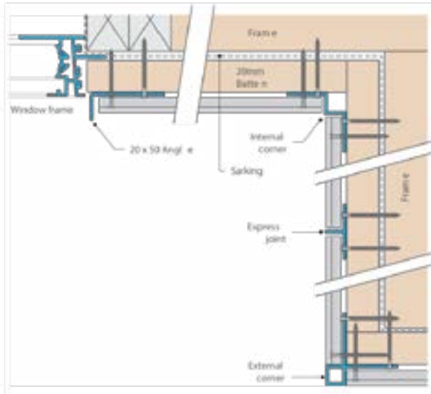
Hidden Interior / external stops (aluminium) extra detail Note: Nail or Screw cladding as specified
