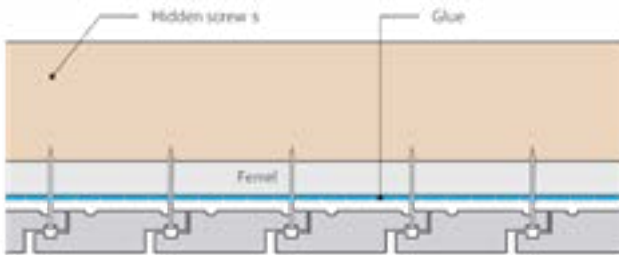
Horizontal installation – internal ceiling
