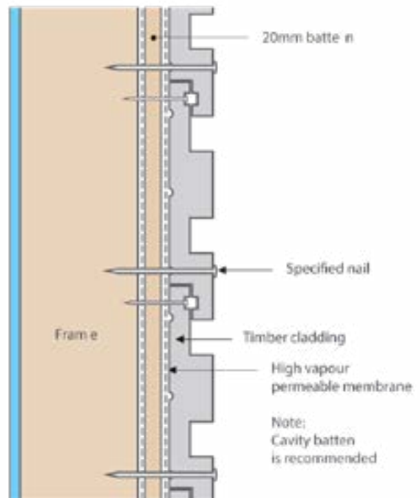
Face fixing showing fixing position
