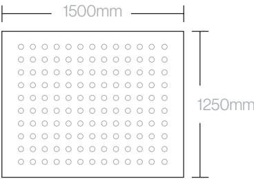
30mm DIA
