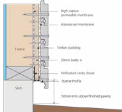
Minimum clearance level of cladding above final ground levels and finishing below bottom plate
